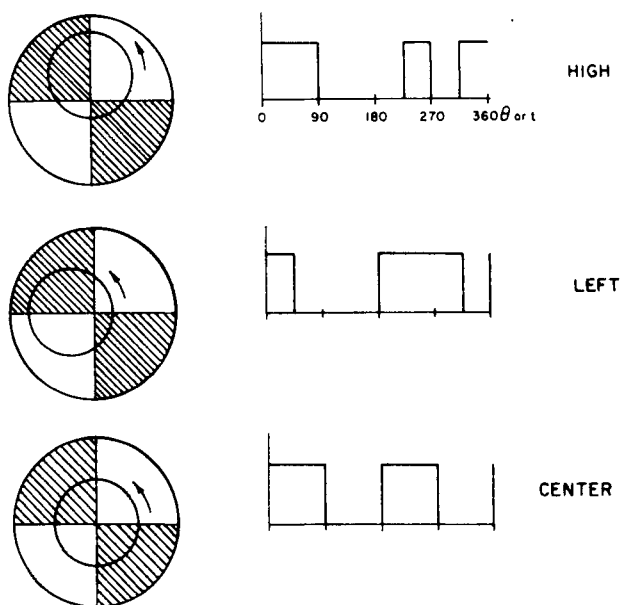
Figure 38. Circular scan x-y tracker.
