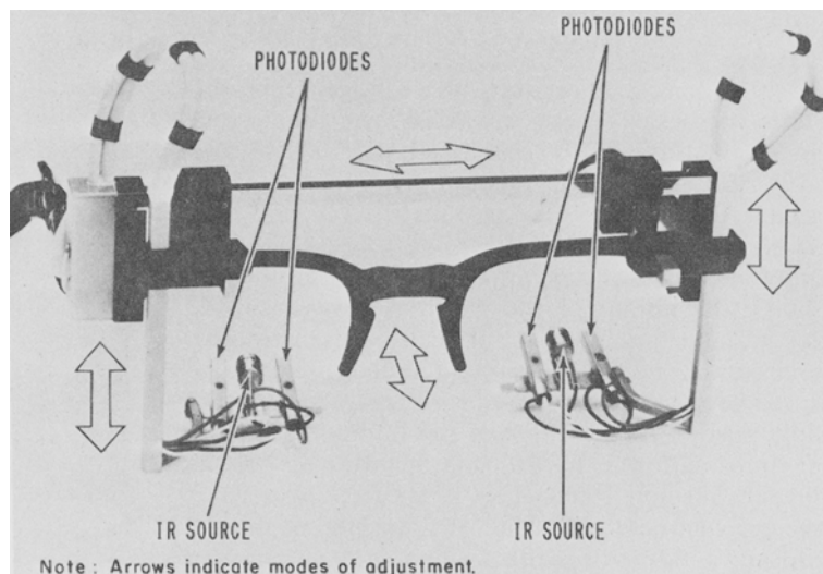
Figure 16. Spectacle mounted differential reflectivity device (Courtesy of Biometrics Division, Narco Bio-Systems, Inc.).
