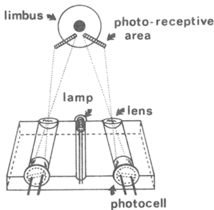
Figure 21. Illumination pattern for two-dimensional limbus tracking (Jones, 1973).
