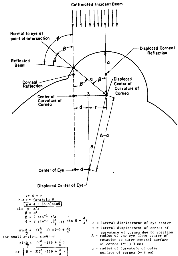
Figure 3. Corneal reflection geometry.
