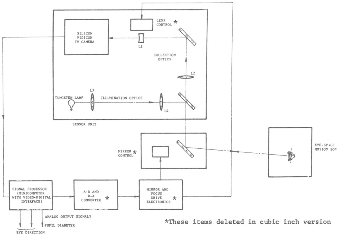
Figure 31. Schematic of the cubic foot remote oculometer (Merchant & Morrisette, 1974).
