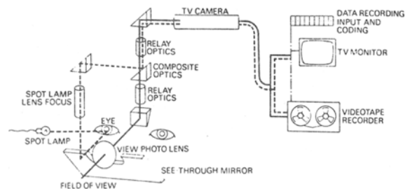
Figure 10. Schematic diagram for head-mounted TV corneal reflex system (Courtesy of Rees Instruments, Ltd.).
